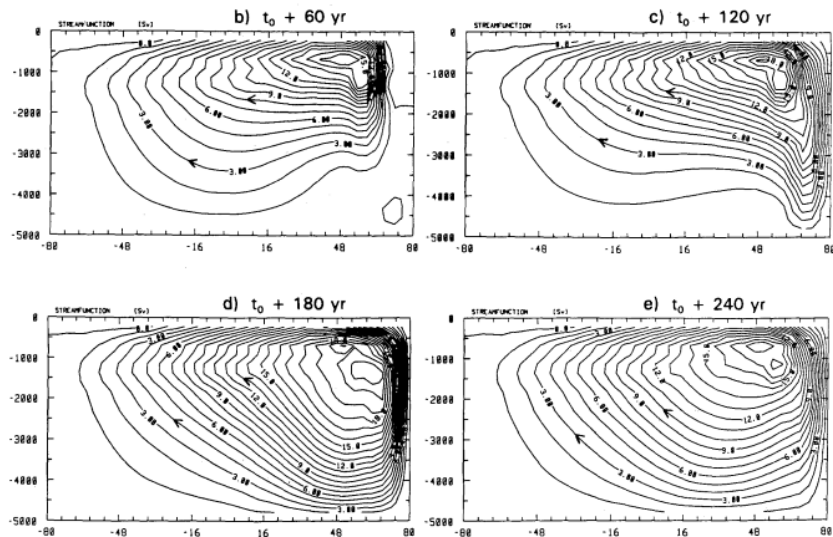
Fig. 3a-e. Streamfunction contours at 60-yr intervals which span the 240-yr oscillation EE' in Fig. 2. a t = 6830 \text{ yr} = t_0 ; b t_0 + 60 \text{ yr} ; c t_0 + 120 \text{ yr} ; d t_0 + 180 \text{ yr} , and e t_0 + 240 \text{ yr} (end of oscillation)
