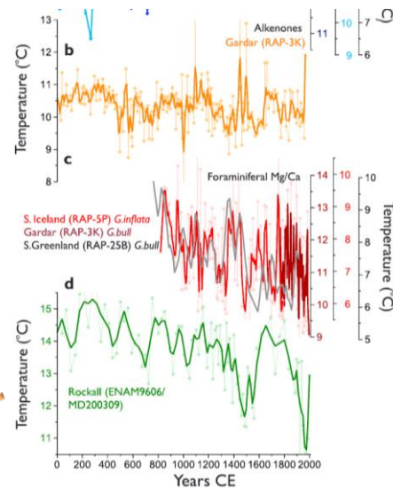
(b) alkenone records from RAPiD-21-3K; (d) foraminiferal Mg/Ca-based temperature reconstructions from Rockall Trough ENAM9606/MD200309
